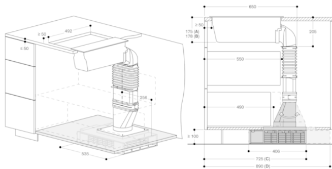
A: Surface mounting B: Flush mounting (only VL414) C: Filter access from the front. Connecting piece flat/round towards the front D: Filter access from the back. Connecting piece flat/round towards the back measurements in mm
